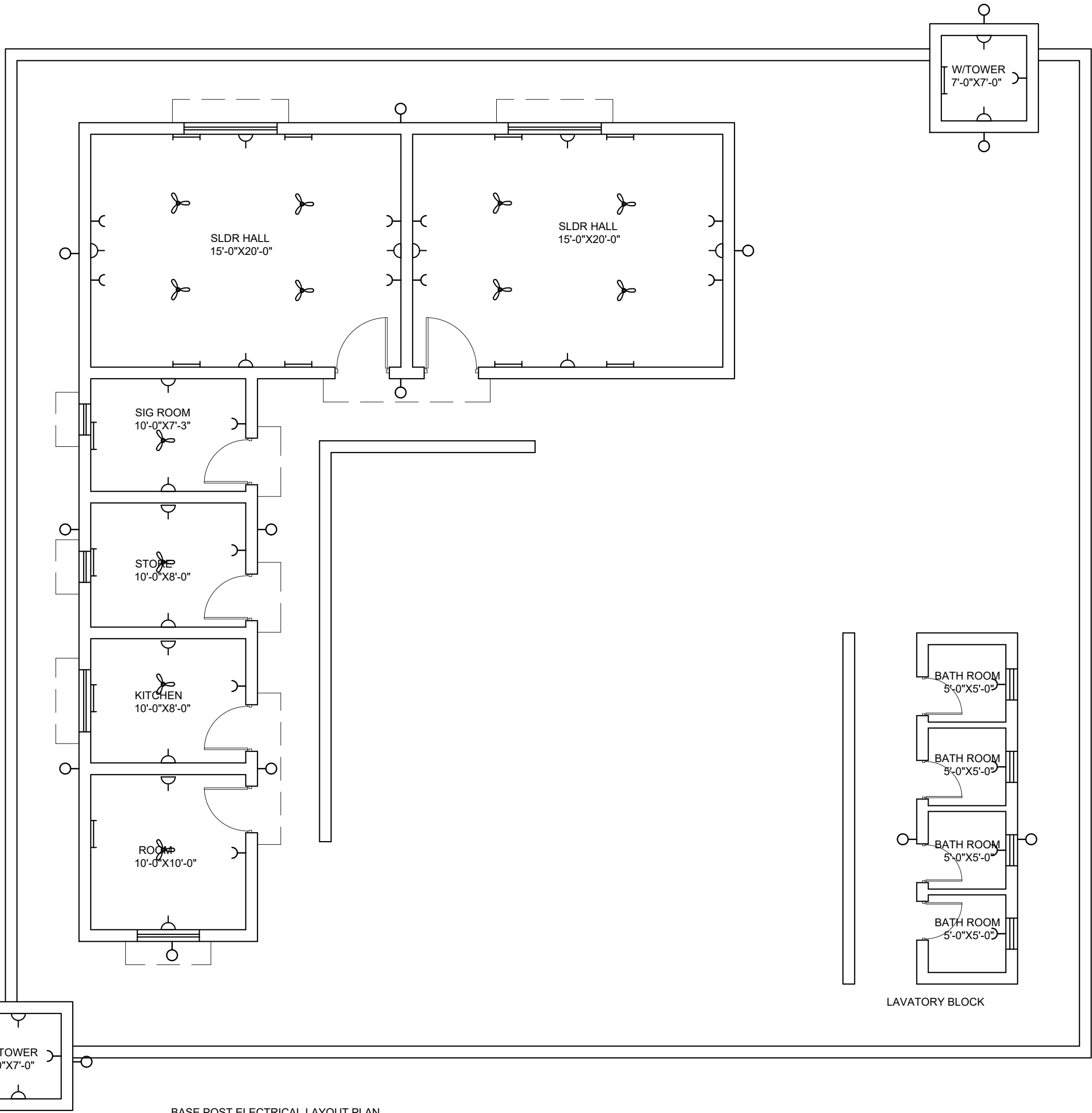
BASE POST ELECTRICAL LAYOUT PLAN
